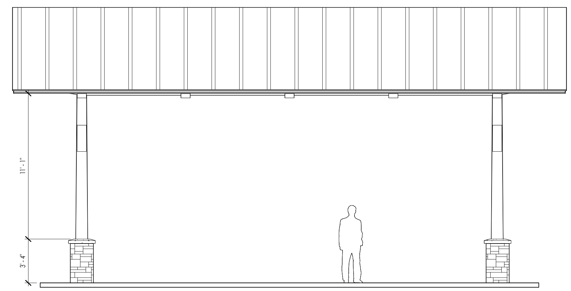
③ BACK ELEVATION - PAVILION 1/4" = 1'-0"
