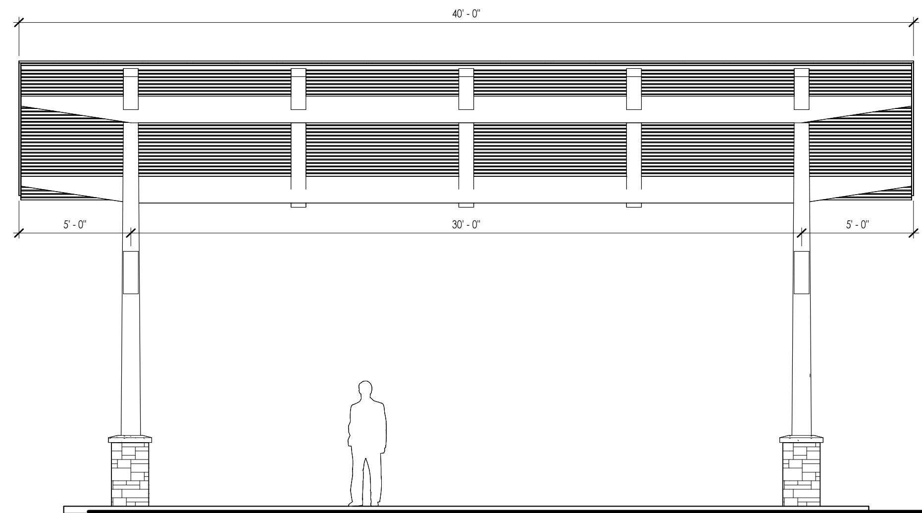
① FRONT ELEVATION - PAVILION 1/4" = 1'-0"
