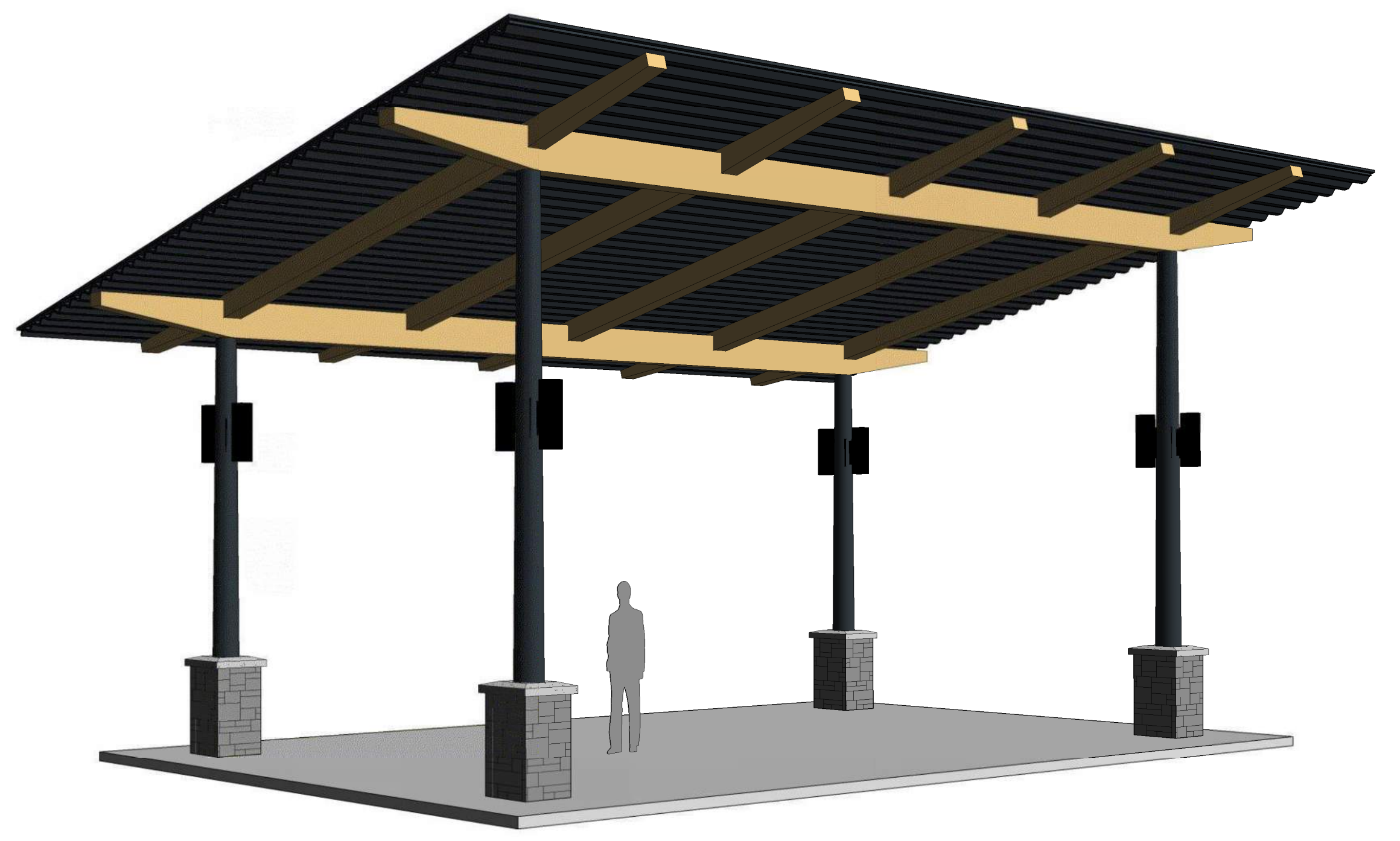
④ PERSPECTIVE - PAVILION
