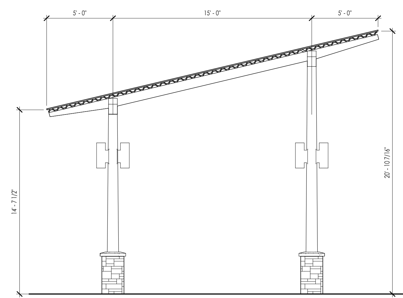
② LEFT ELEVATION - PAVILION 1/4" = 1'-0"
